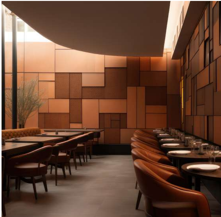
Wall textures
